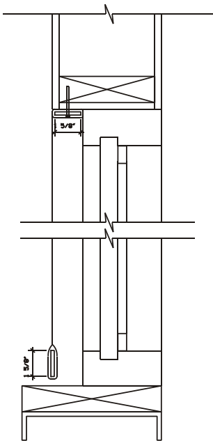
INSIDE MOUNT
